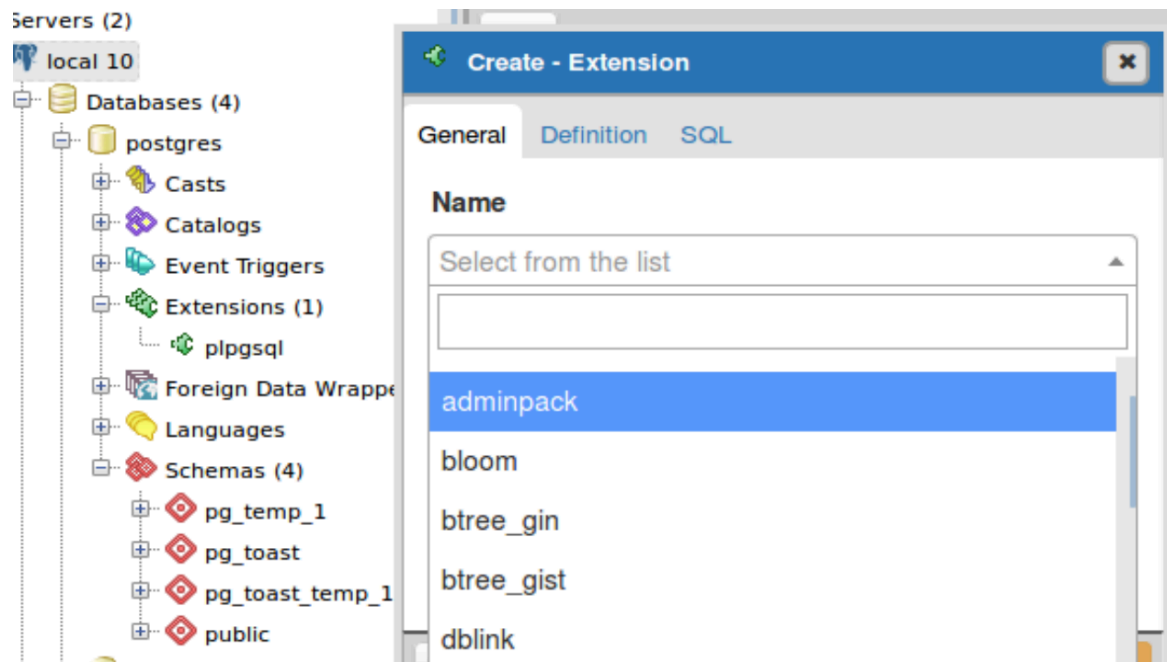
Figure 4-6. Installing extensions using pgAdmin4
