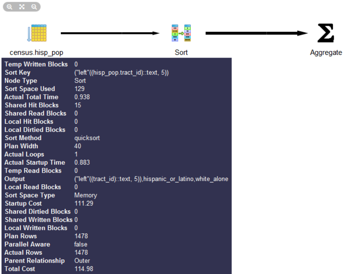
Figure 4-17. Graphical explain example
