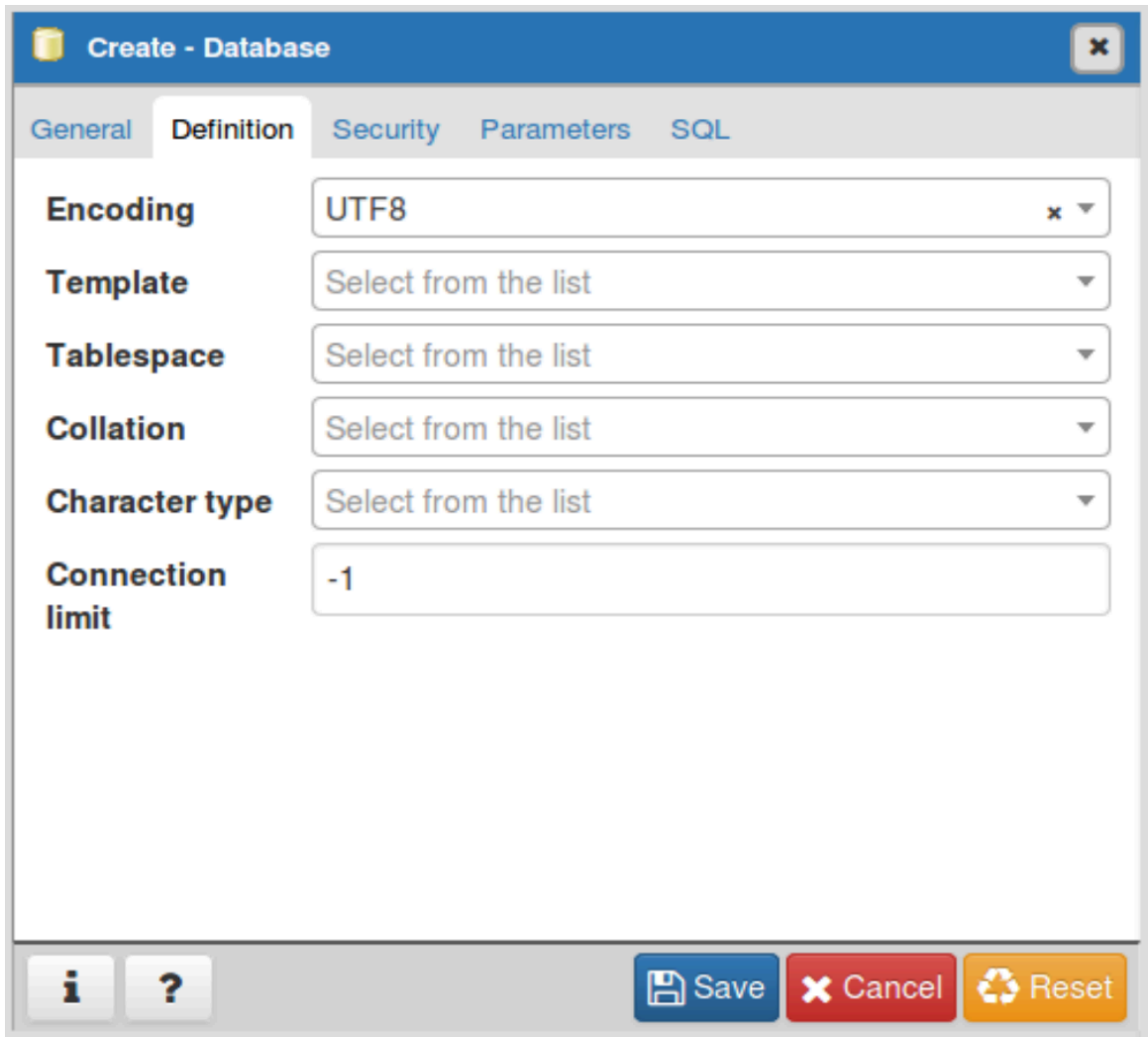
Figure 4-7. Creating a new database in pgAdmin4
